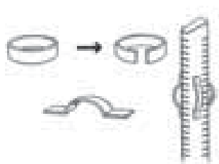
Self made spacer rings attached to the filter screen
